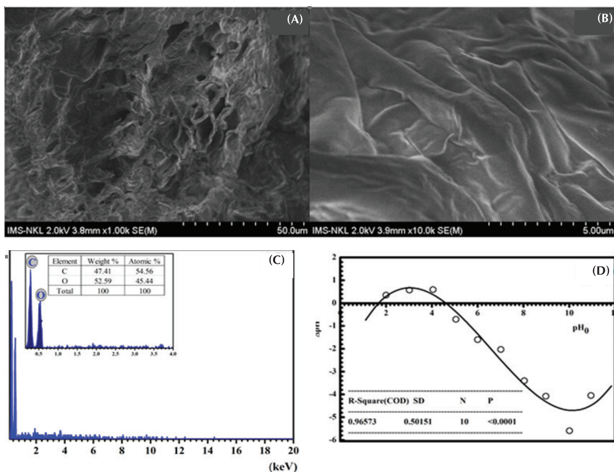
Fig. 1. (A, B) SEM images at different magnifications, (C) the EDX spectrum, and (D) pH ZPC of the pomelo fruit peel.
