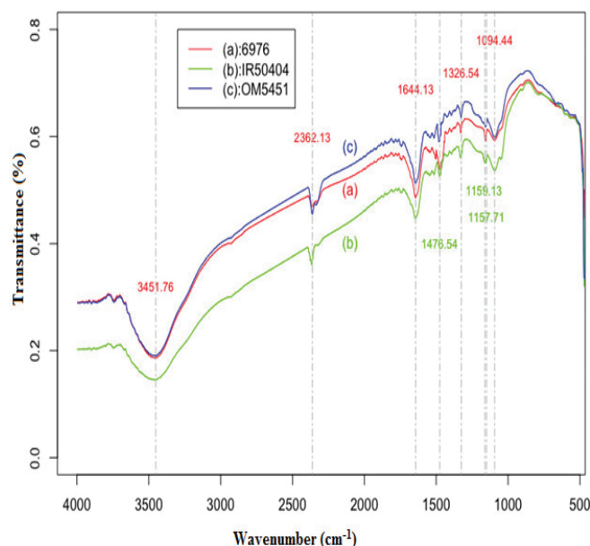
Fig. 2. FTIR spectra of hemicellulose extracted from rice straw.
