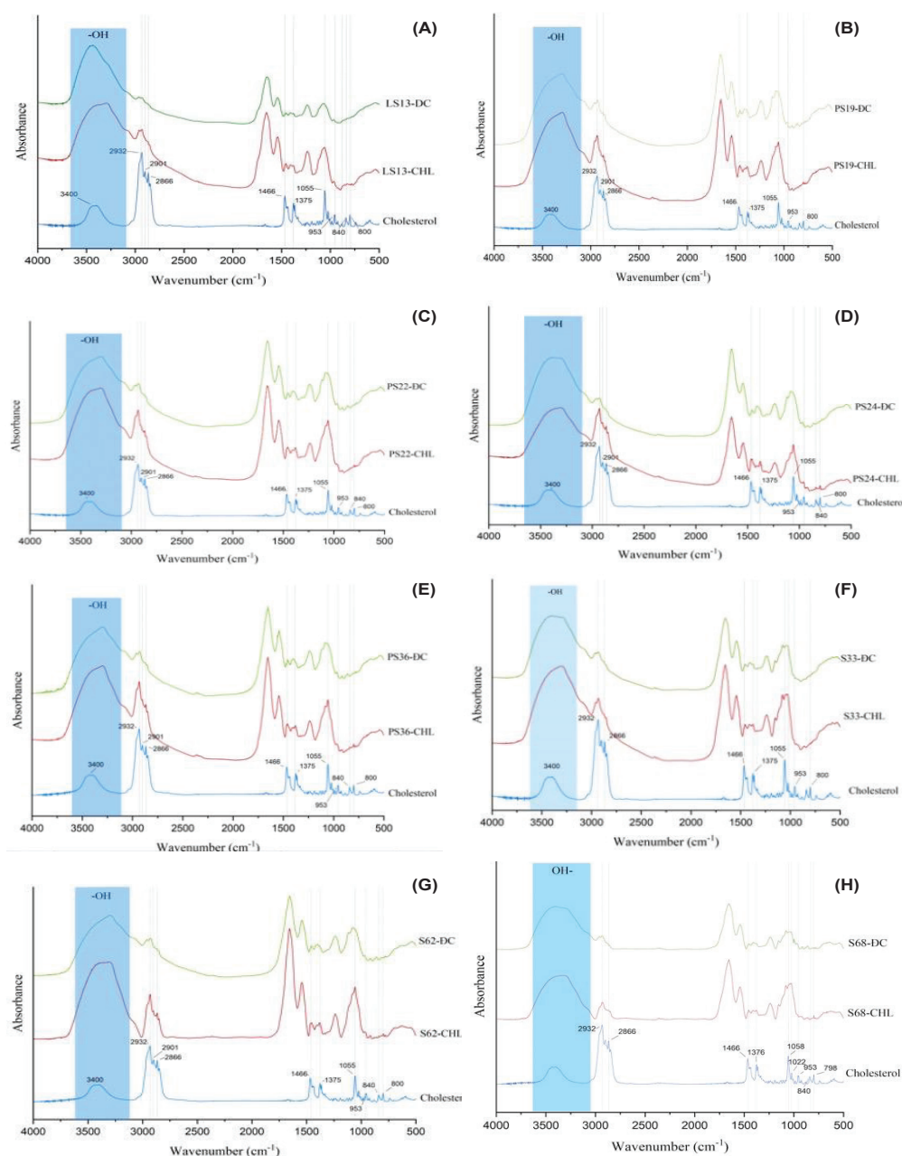
Fig. 4. The FTIR spectra of bacterial strains cultured in media with and without cholesterol supplementation compared to standard cholesterol. (A) LS13; (B) PS19; (C) PS22; (D) PS24; (E) PS36; (F) SMB33; (G) SMB62; (H) SMB68. Source: Proposed by the authors.
