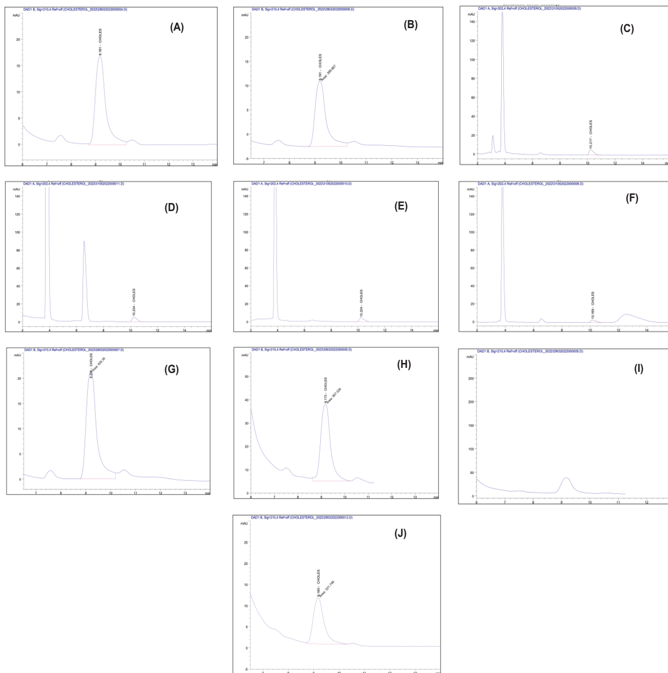
Fig. 7. HPLC chromatograms showing the cholesterol content of SMB33 (A), LS13 (B), PS22 (C), SMB62 (D), PS36 (E), PS19 (F), PS24 (G), SMB68 (H), L. brevis strain - strain control (I), and cholesterol standard (J). Source: Proposed by the authors.
