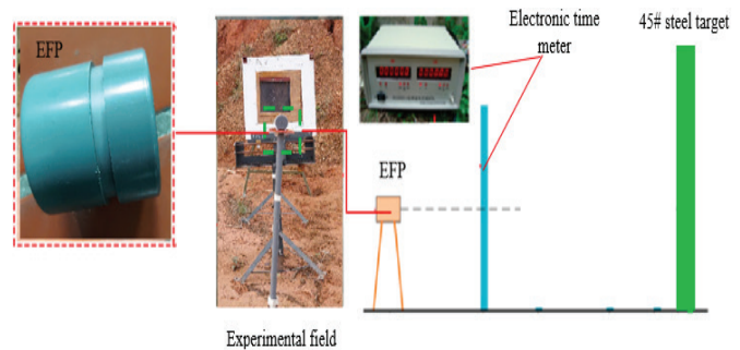
Fig. 4. Experimental measurement of EFP velocity and penetration depth. Source: Proposed by the authors.
