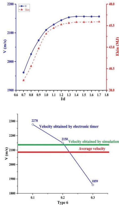
Fig. 6. Velocity of EFP obtained by simulation and experiments. Source: Proposed by the authors.
