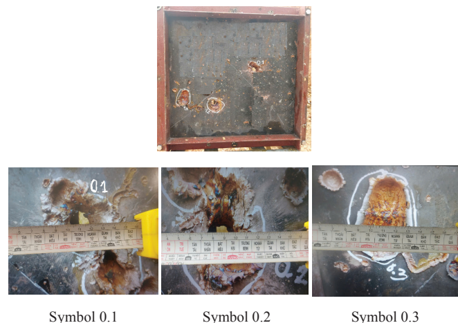
Fig. 5. Experimental results of EFP interaction with steel plate. Source: Proposed by the authors.
