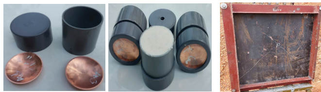
Fig. 3. EFP and steel target. Source: Proposed by the authors.
