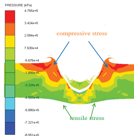
Fig. 7. Steel target plate subjected to EFP impact. Source: Proposed by the authors.
