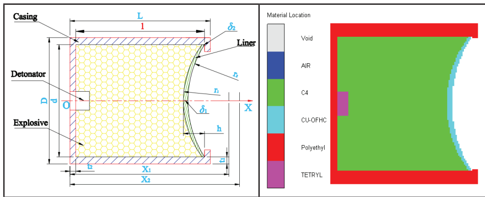
Fig. 1. EFP model and simulation model in ANSYS Autodyn. Source: Proposed by authors.
