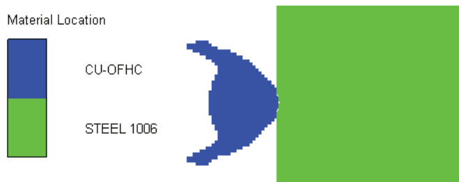
Fig. 2. Simulation of EFP impact on steel plate. Source: Proposed by the authors.
