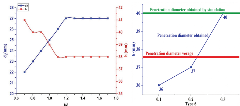
Fig. 8. Diameter and depth of EFP obtained by simulation and experiments. Source: Proposed by the authors.
