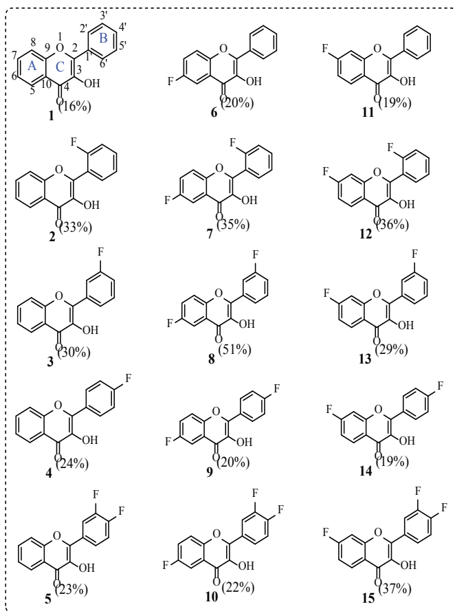
Fig. 2. Chemical structures of fluorinated flavonols (1-15) synthesised by the AFO reaction. The isolated yields are in parentheses.
