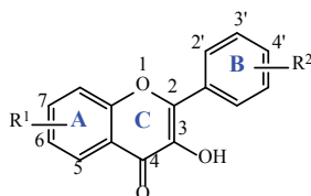
Fig. 1. Skeleton of flavonols [1].
