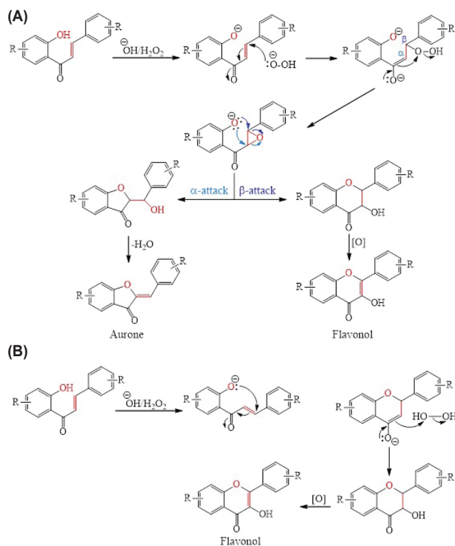
Scheme 2. Two proposed mechanisms of the AFO reaction for the flavonol synthesis [10]. (A) The first possible reaction mechanism suggested that the chalcone epoxide serves as a key intermediate; (B) The second hypothesis proposed that the formation of 3-hydroxyflavanone starts with the cyclisation of the phenolate ion at the \beta -position.
