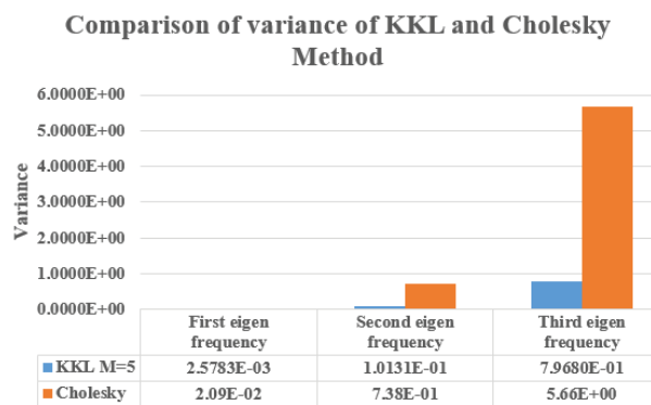
Fig. 16. Comparison of variance of eigenfrequency by Monte Carlo simulations with Cholesky decomposition and Monte Carlo simulations with Kosambi-Karhunen-Loève expansion.
