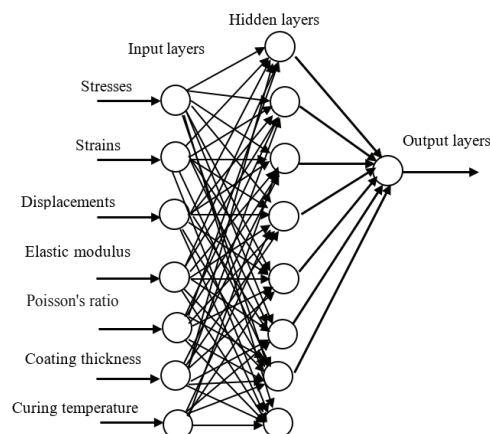
Fig. 5. Schematic diagram of ANN method for predicting residual stresses.
