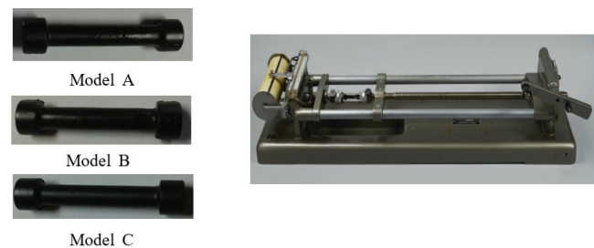
Fig. 3. Epoxy coating specimens for tensile testing and tensile testing machine.
