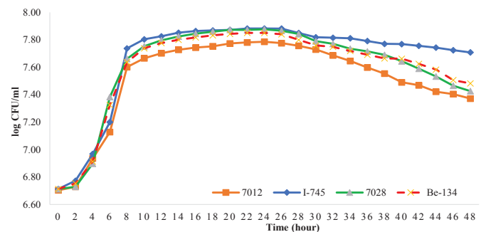
Fig. 1. Growth curves of the four yeast strains in pretreated SRH.
