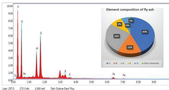
Fig. 4. Chemical composition of fly ash by EDX technique.
