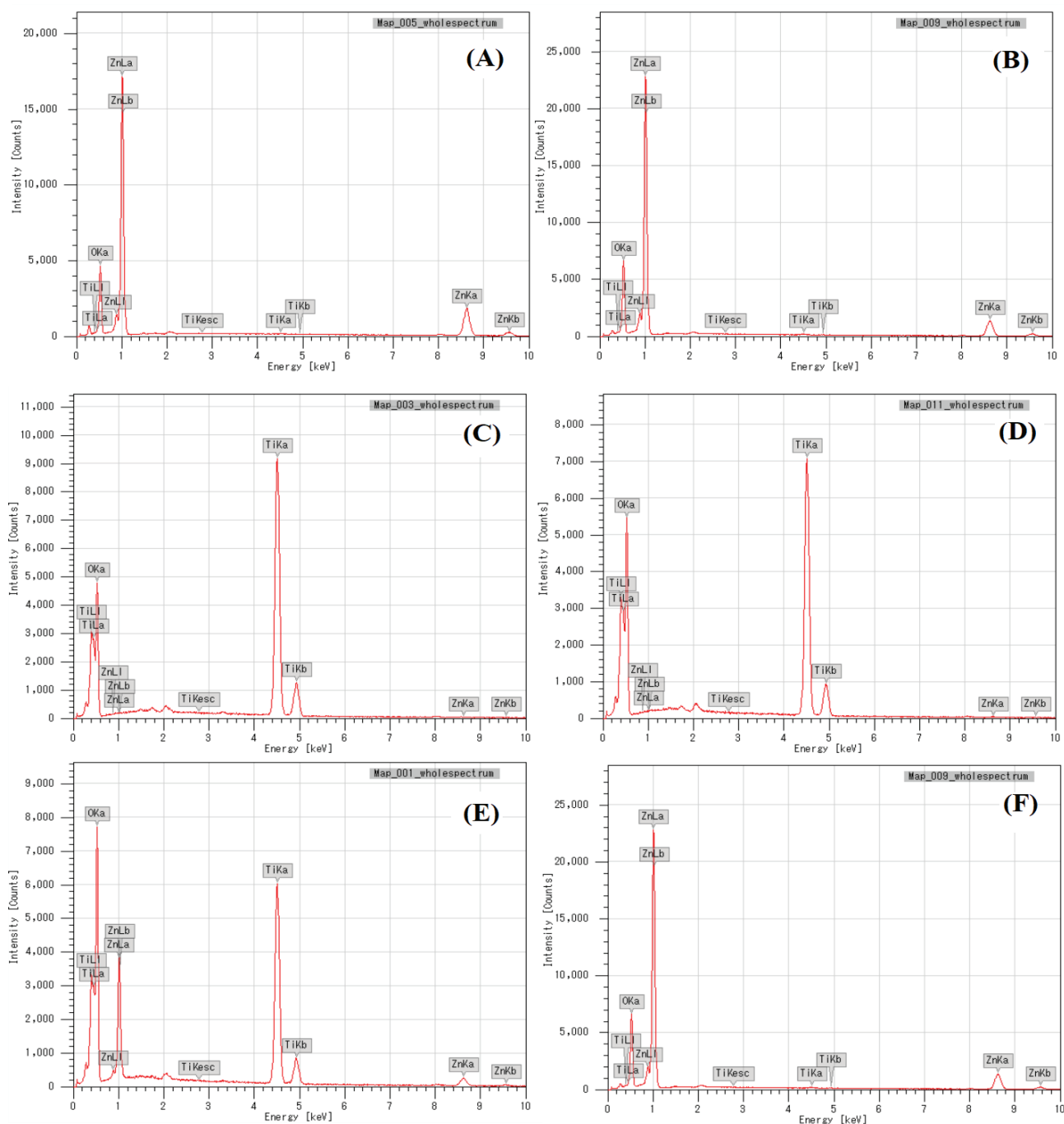
Fig. 4. EDX spectra of photocatalysts before and after reaction: (A, B) ZnO, (C, D) \text{TiO}_2 , and (E, F) 10\%\text{ZnO}@ \text{TiO}_2 .
