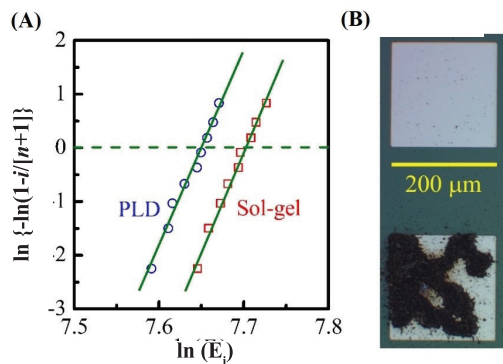
Fig. 5. (A) Weibull distribution of breakdown strength for the capacitors of PLZT thin films deposited by sol-gel and PLD and (B) optical images of thin film capacitors before (upper) and after breaking (lower).
